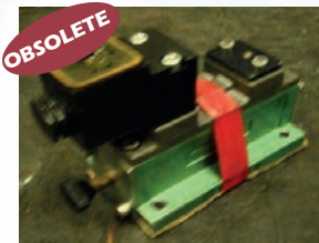
Numatics® Mark 6 electrical single op.
